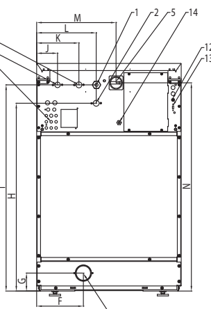
Traseira
